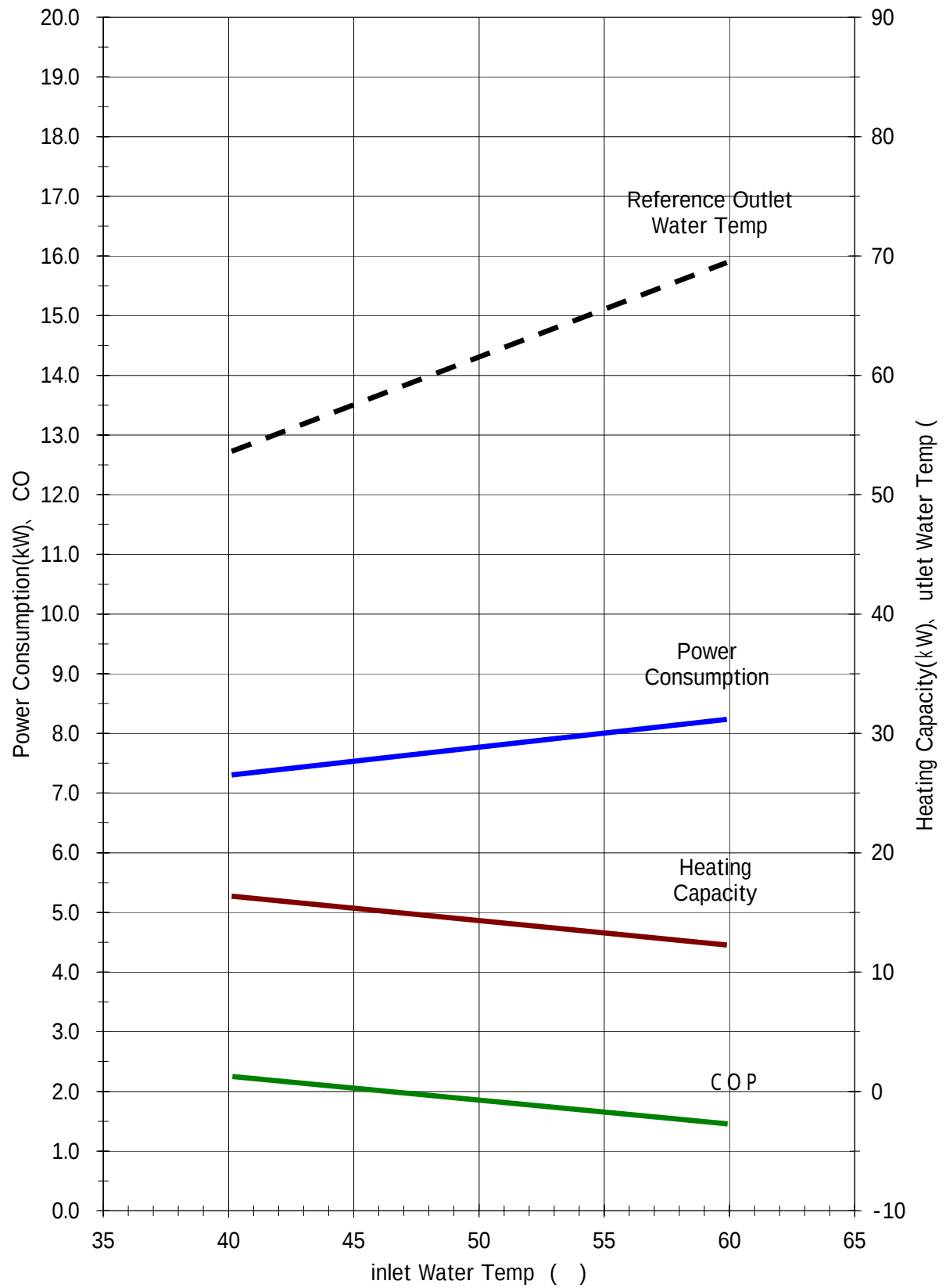
Circulating Operation ( 6.0Hz, Air Temp2 )
