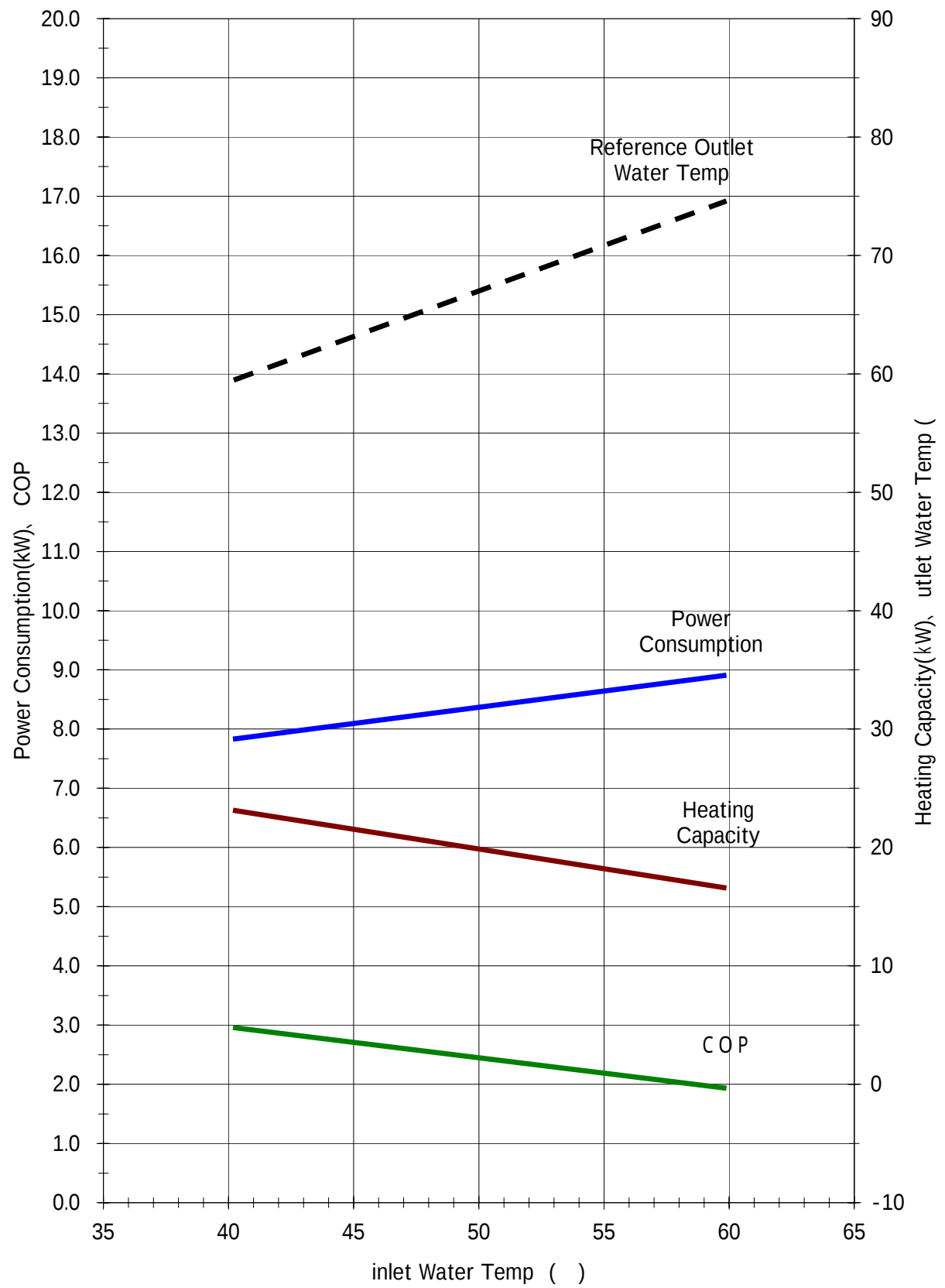
Circulating Operation ( 6.0Hz, Air Temp 16 )
