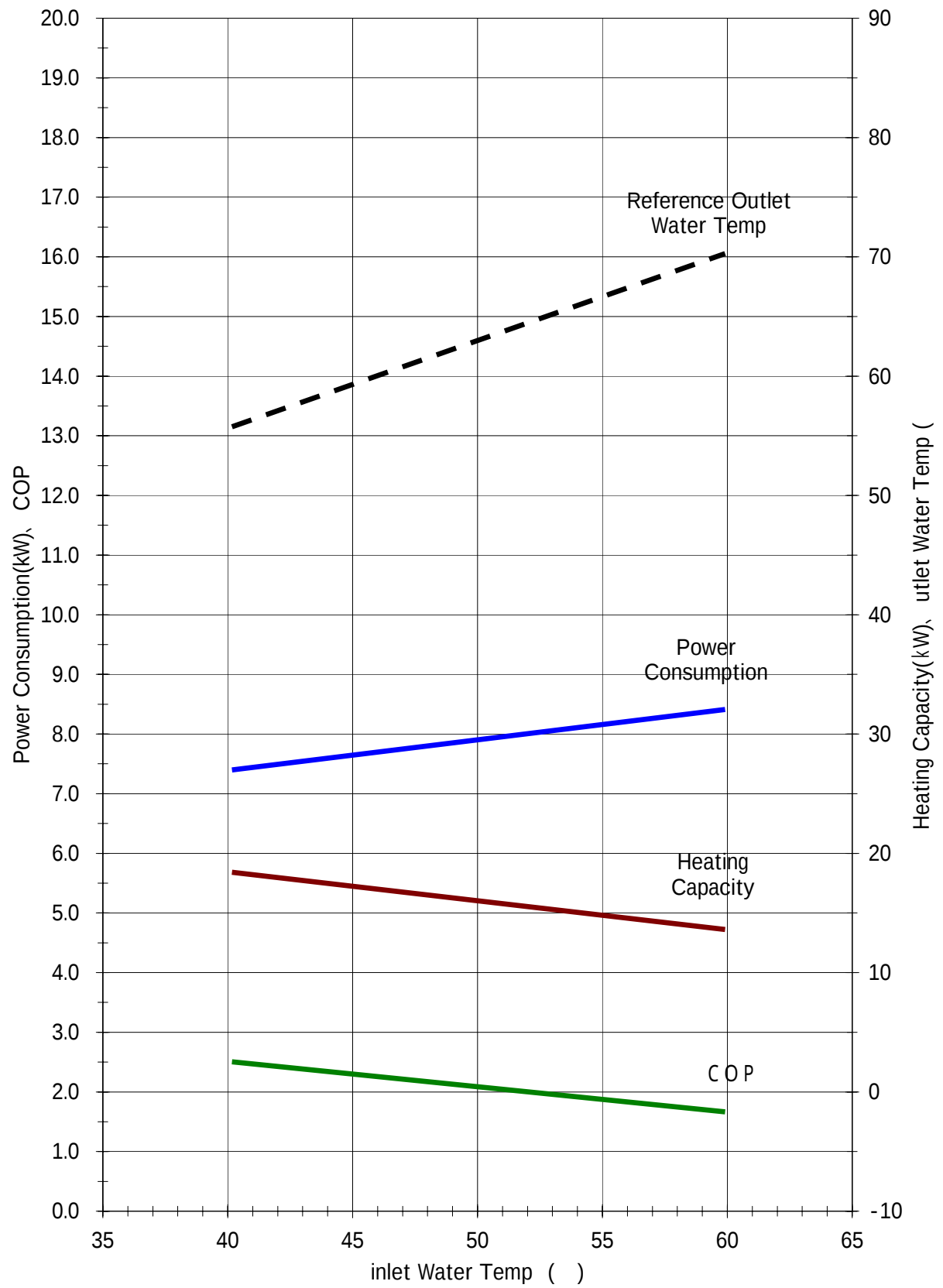
Circulating Operation ( 6.0Hz, Air Temp 7 )
