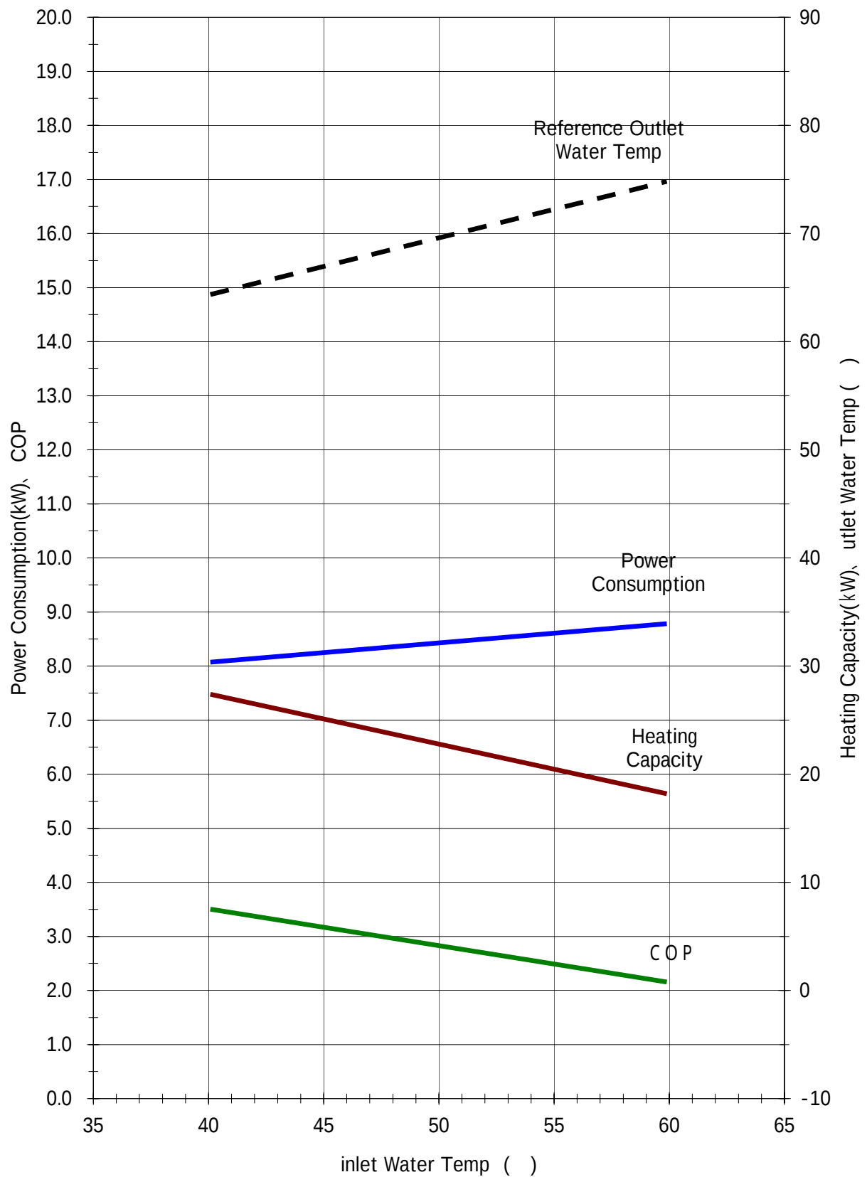
Circulating Operation ( 6.0Hz, Air Temp 25 )
